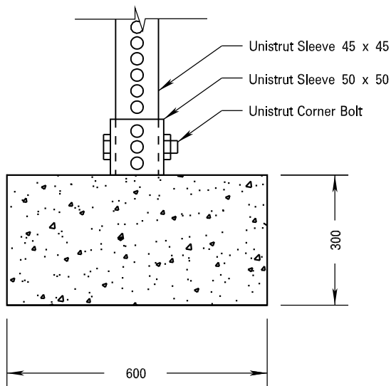
TRAFFIC SIGN TEMPORARY STAND
