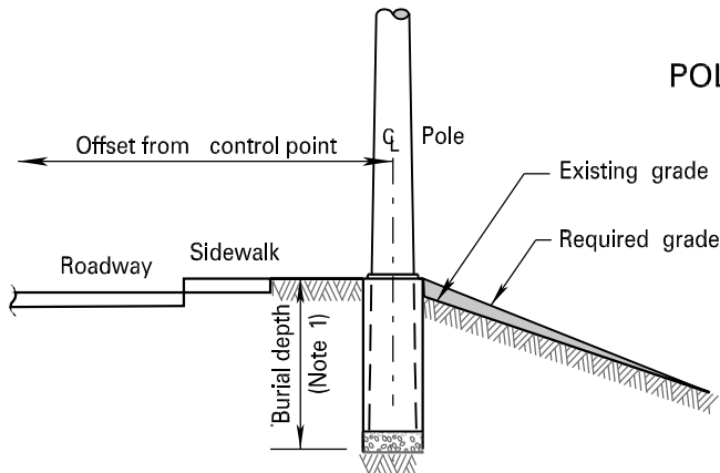
POLE FOUNDATION IN FILL
