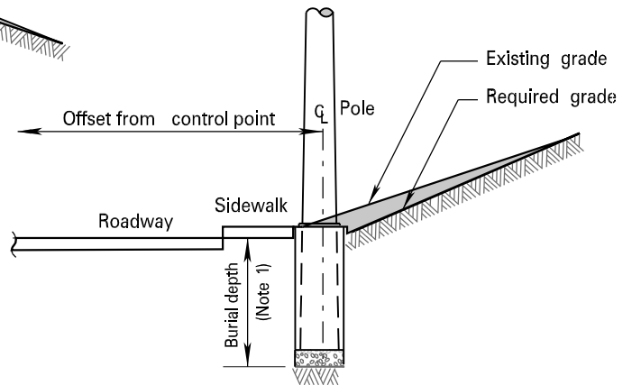
POLE ADJACENT TO SIDEWALK
