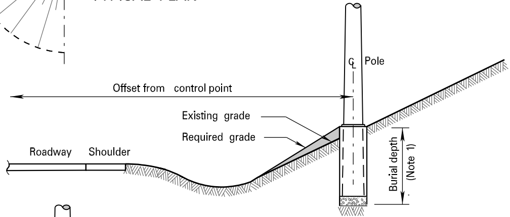
POLE FOUNDATION IN CUT
