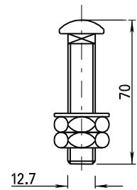
ADJUSTING BOLT
