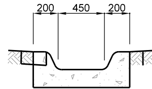
SECTION Z - Z
