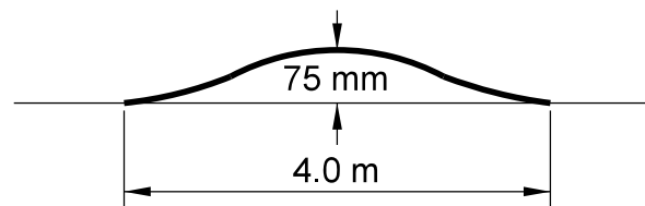
SECTION A - A SINUSOIDAL SPEED HUMP
