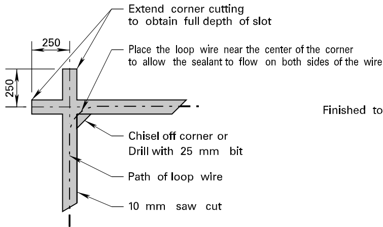
DETAIL 'B' (TTD 810.005)
