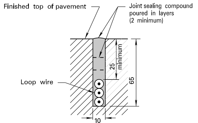
SECTION B-B (TTD 810.005)
