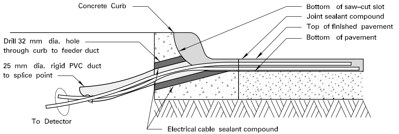
DETAIL 'A' (TTD 810.005)
