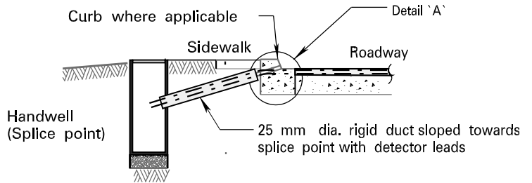
SECTION A-A (TTD 810.005)
