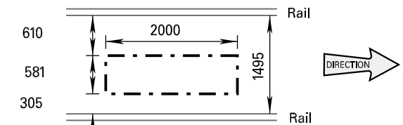
DIPOLE LOOP INSTALLATION DETAIL BETWEEN STREETCAR TRACKS
