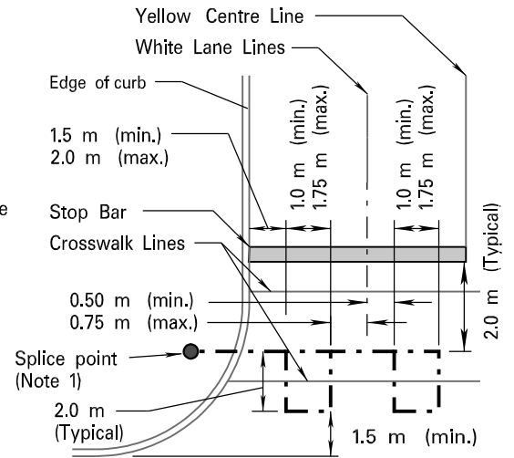
PRIORITY CANCEL LOOP INSTALLATION DETAIL
