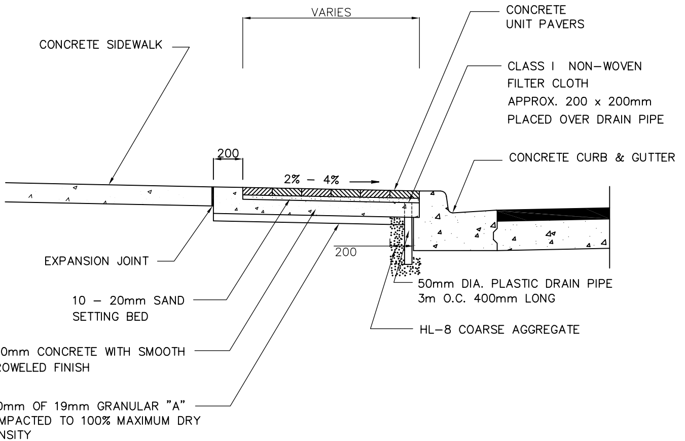
SECTION A
