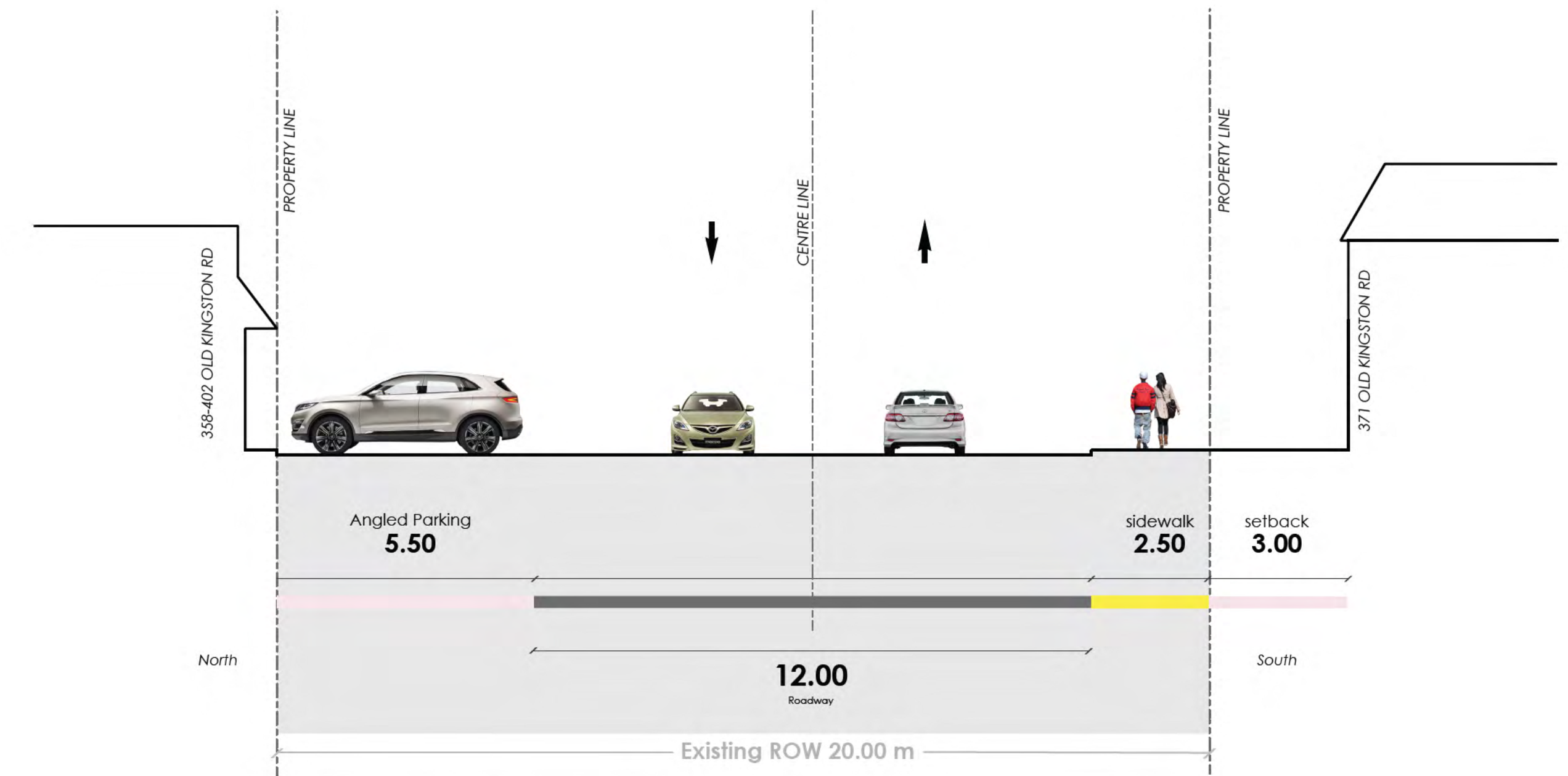
EXISTING OLD KINGSTON ROAD TYPICAL SECTION (east of Morrish Road intersection)
