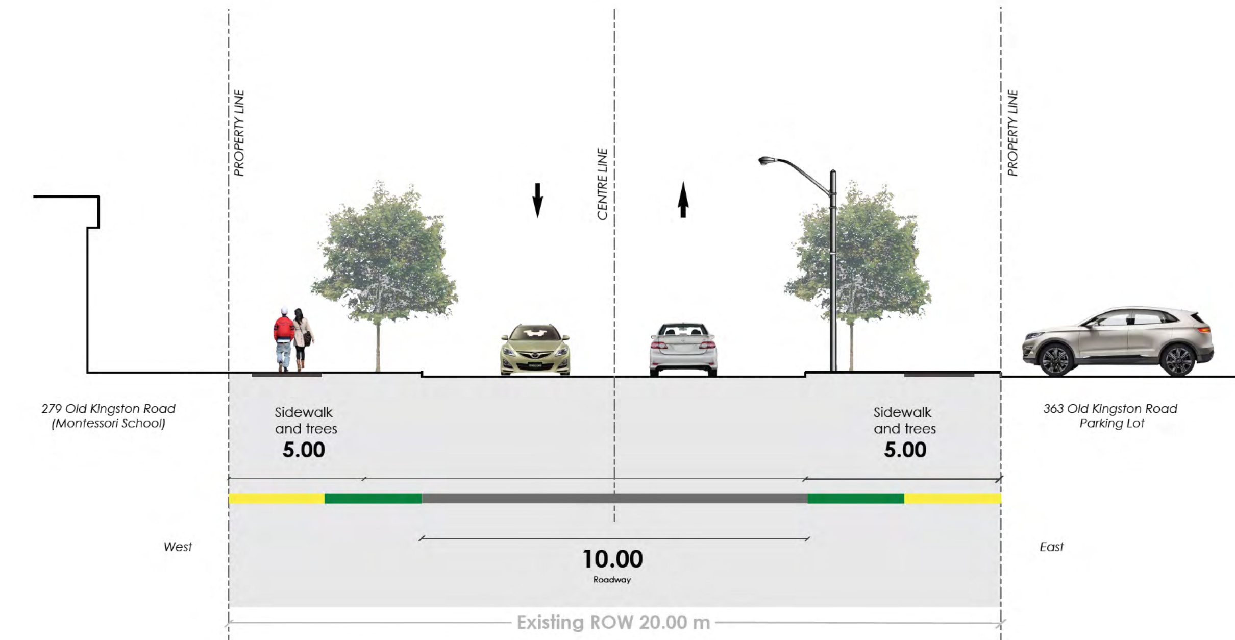
EXISTING MORRISH ROAD TYPICAL SECTION (south of Old Kingston Road intersection)
