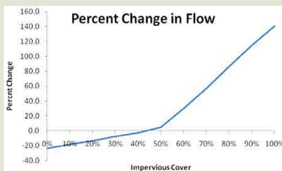
Figure 29. Percent change in flow given varying percent impervious cover in Don watershed
