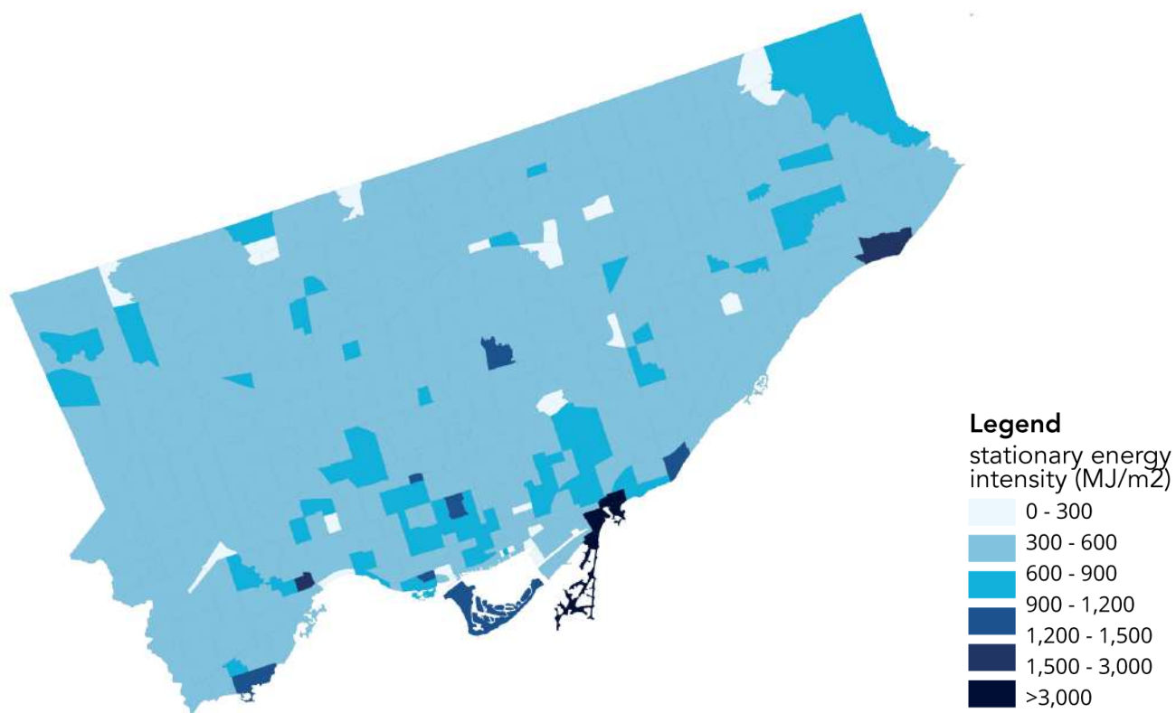
Figure 13. Building energy intensity (MJ/m²), Low Carbon 2050.
