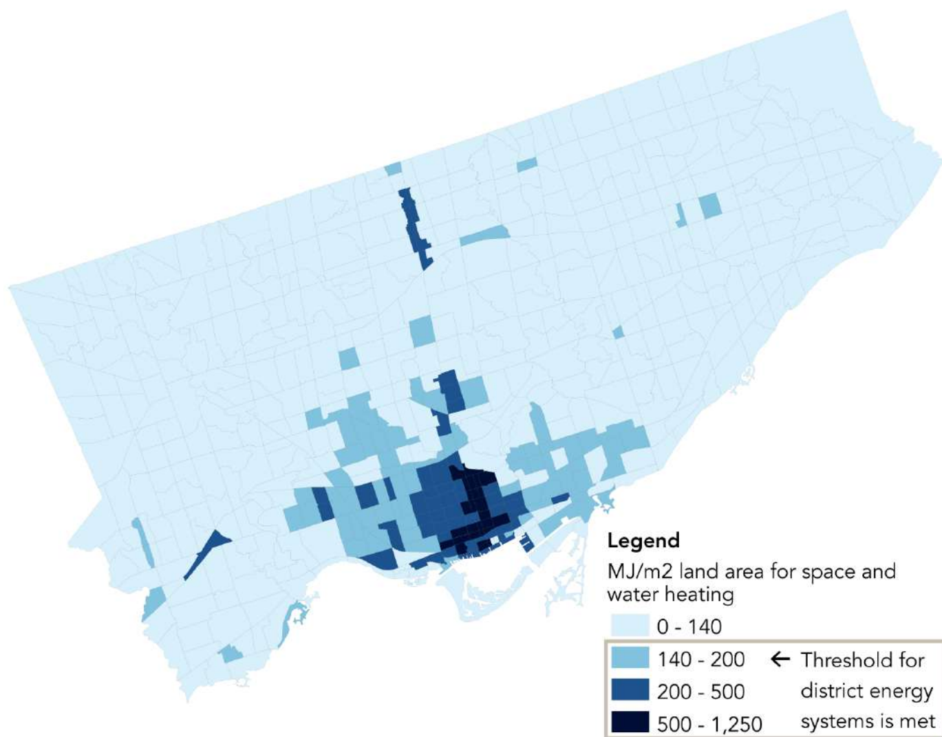
Figure 17. Zones identified in the modelling that meet or exceed the 140 MJ/m 2 threshold for district energy in the 2050 LCS.
