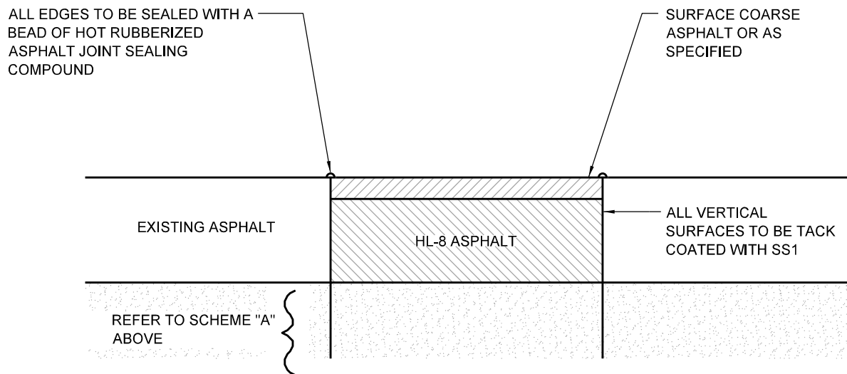
SCHEME B ALTERNATIVE ASPHALT PATCHING
