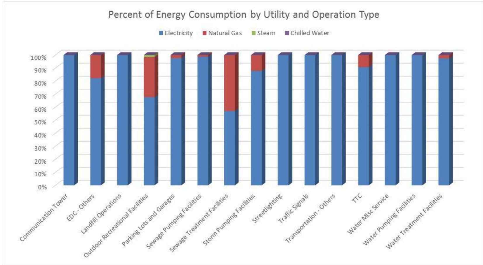
Figure 10: Process Energy Consumption by Utility and Operation Type
