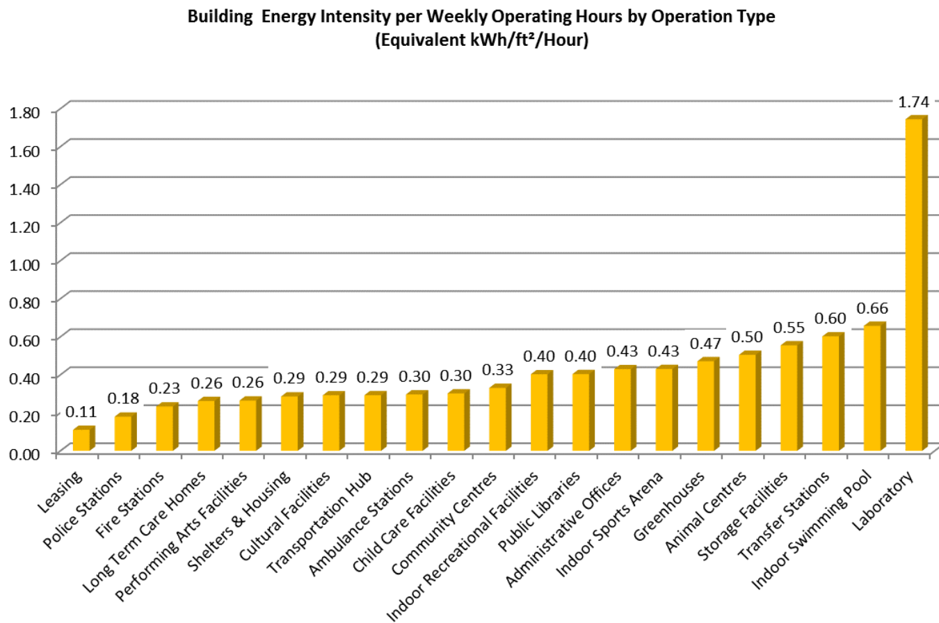
Figure 5: Average Building Energy Intensity per Weekly Operating Hours
