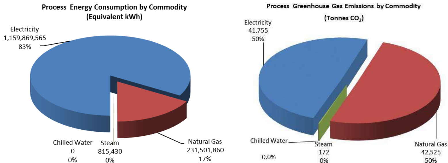
Figure 8: Process Energy Consumption and GHG Emissions by Energy Type
