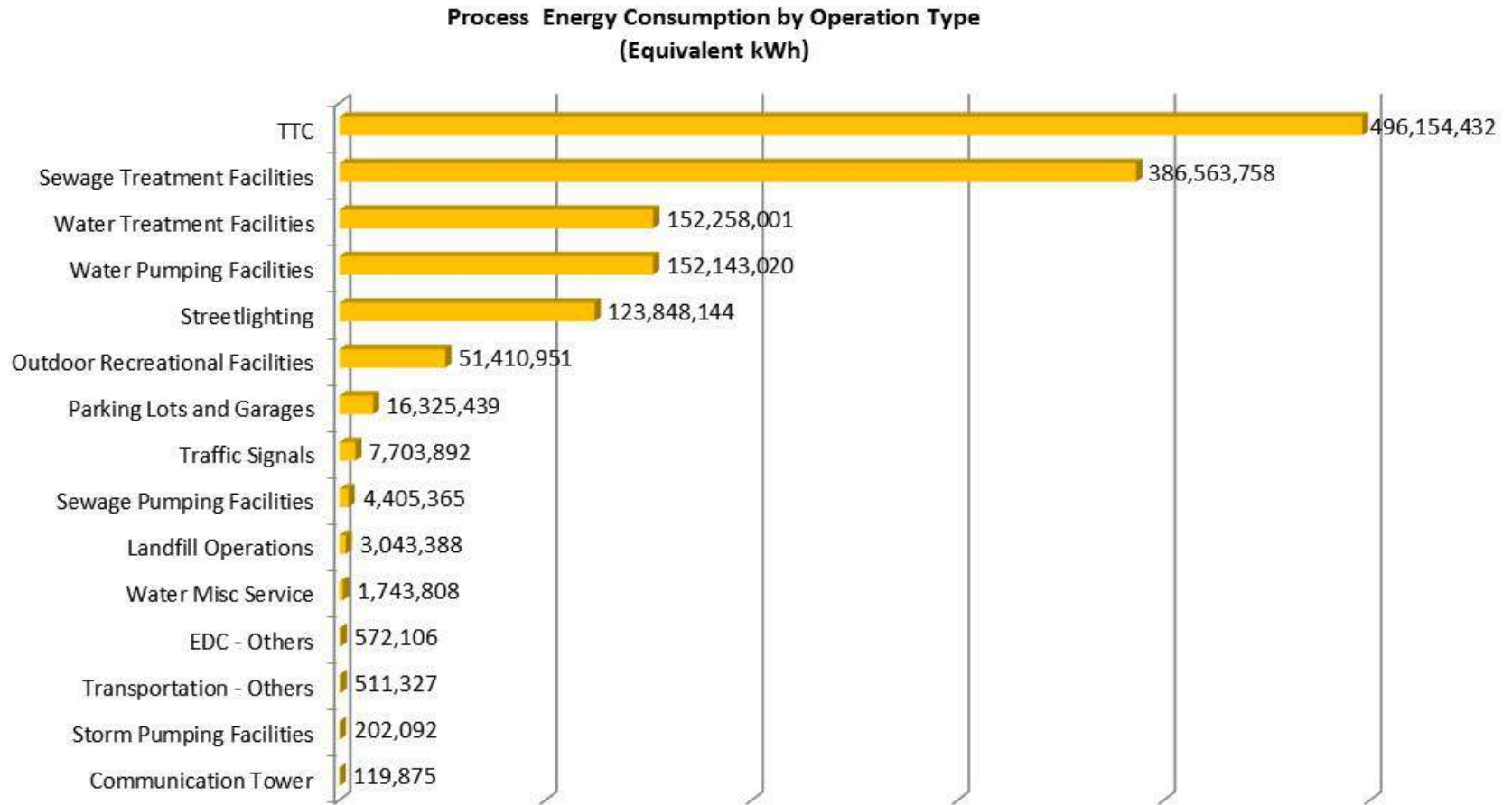
Figure 9: Process Energy Consumption by Operation Type
