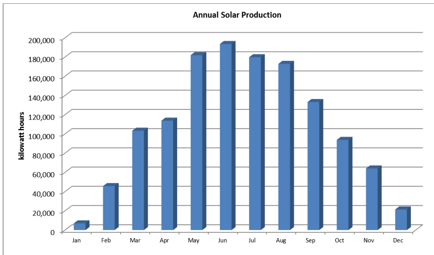
Figure 14: Total Monthly Solar Production
