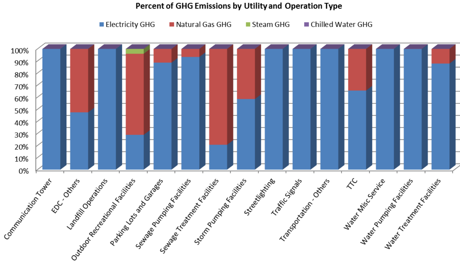
Figure 12: Process-Based Greenhouse Gas Distribution by Operation Type
