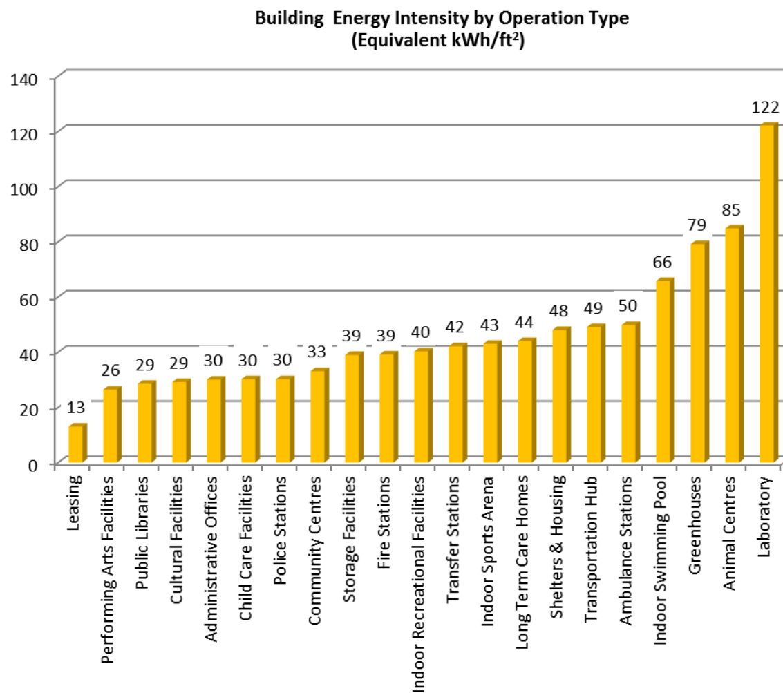
Figure 4: Building Energy Intensity per Operation Type
