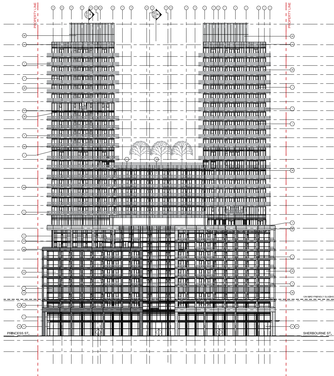
North elevation
