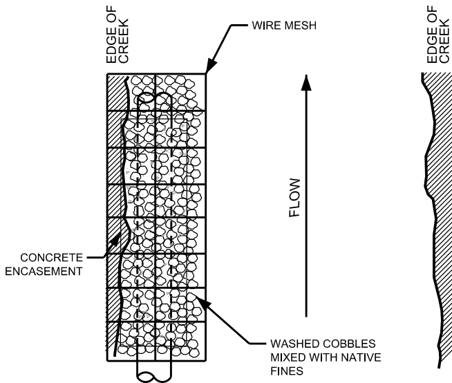
PLAN VIEW (NTS) A
