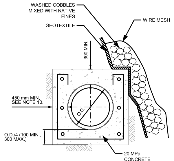
DETAIL VIEW (NTS) C
