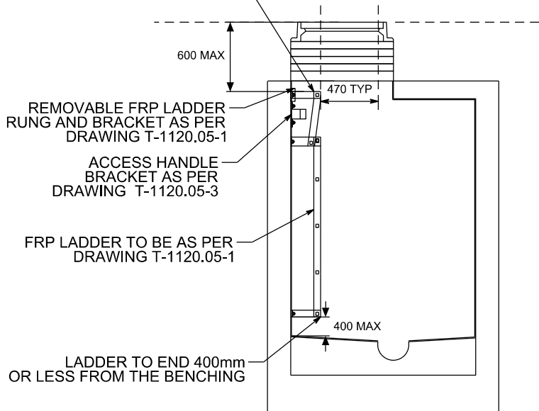
SECTION VIEW (NTS)
