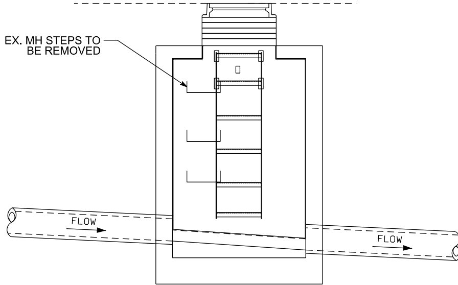
SECTION VIEW (NTS)
