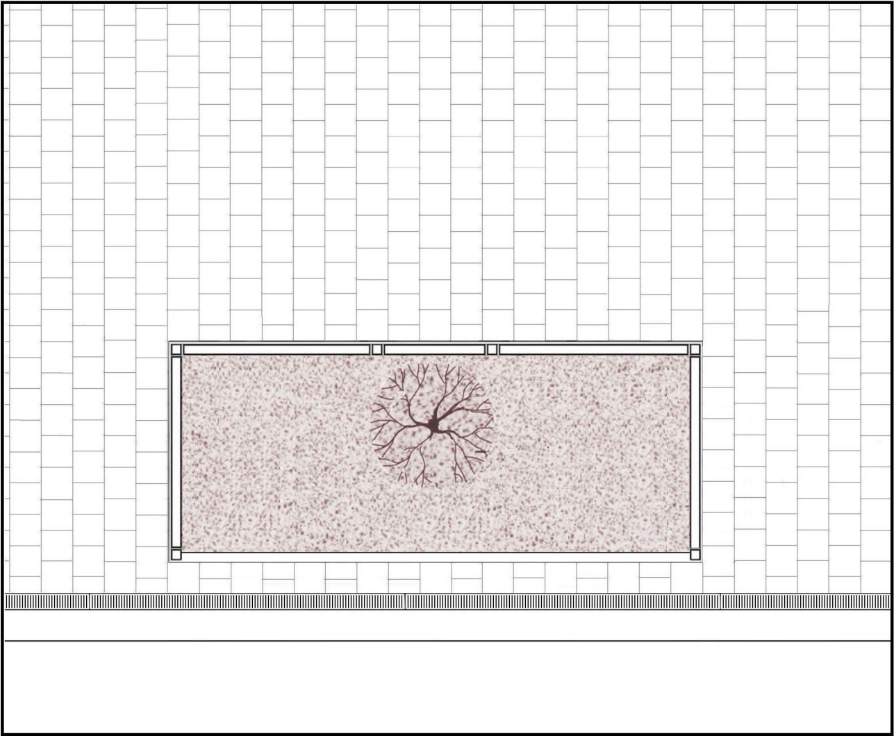
1200 x 3400 wide open planting bed with iron fence T - PCP 3.0
