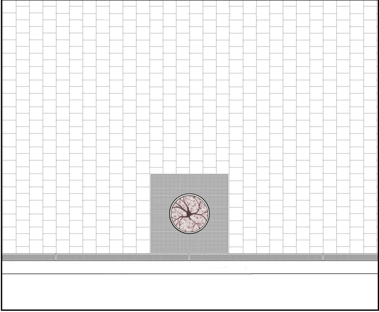
1200 x 1200 in-ground pit with metal tree plate and guard T - PCP 6.0
