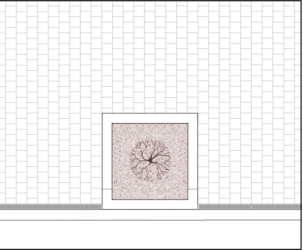
1800 x 1800 raised planting bed with concrete or stone surround T - PCP 2.0
