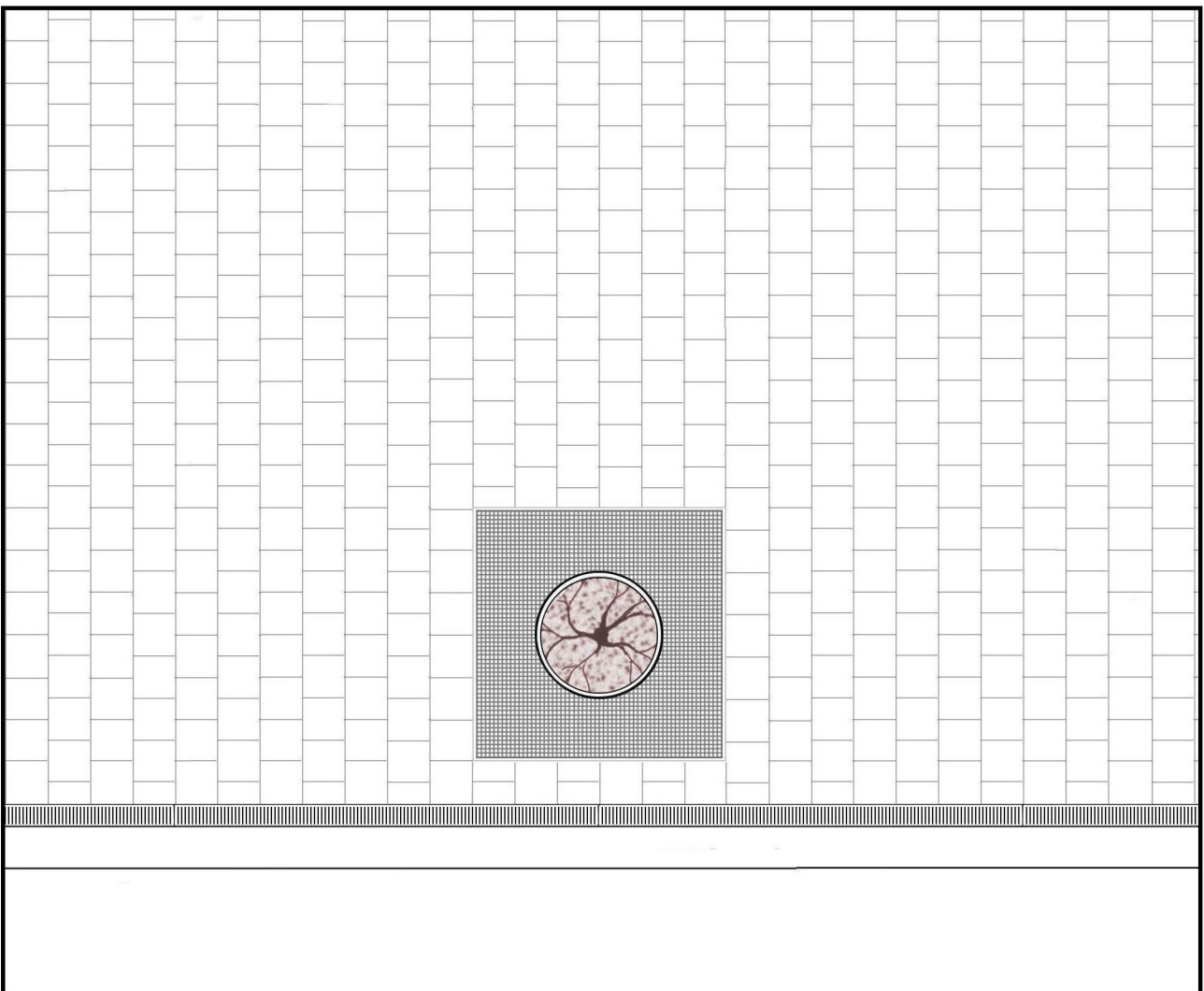
1200 x 1200 in-ground pit with metal tree plate and guard T - PCP 5.0
