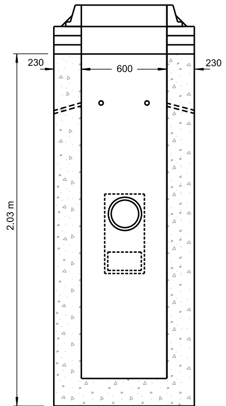
SECTION B
