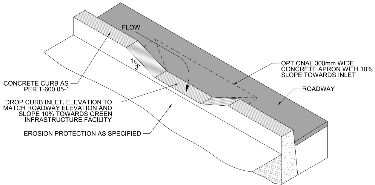
ISOMETRIC VIEW
