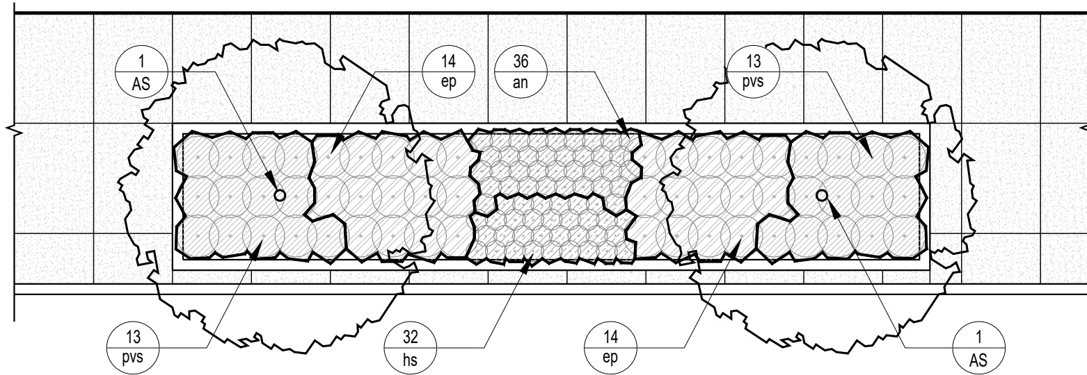
Bioretention Sample Layout 2
