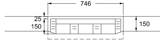
CURB ELEVATION
