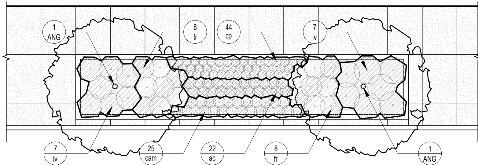
Bioretention Sample Layout 1
