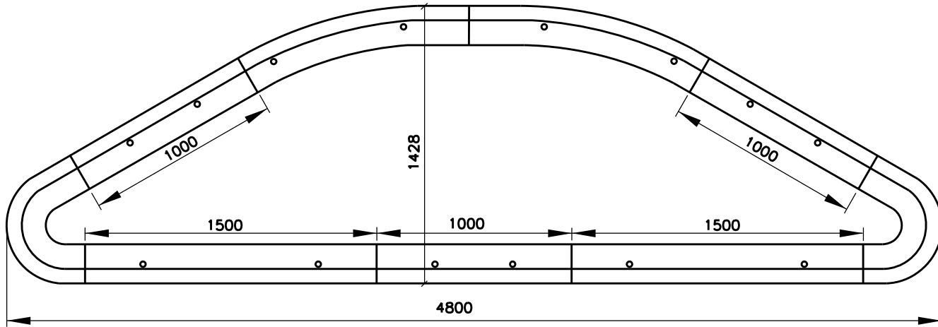
CURBSTONE ISLAND - TYPE C
