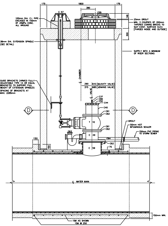
SECTION A
