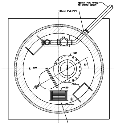
SECTION D
