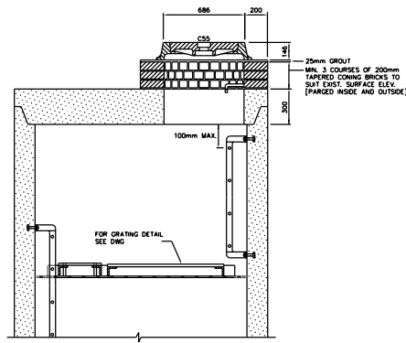
SECTION C
