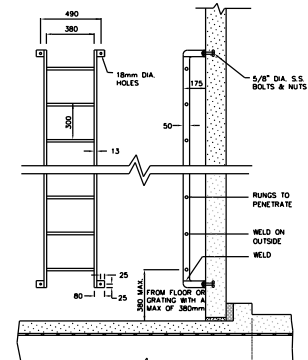
REMOVABLE ALUMINUM LADDER NOT TO SCALE
