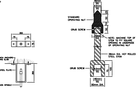
DETAIL OF EXTENSION SPINDLE NOT TO SCALE
