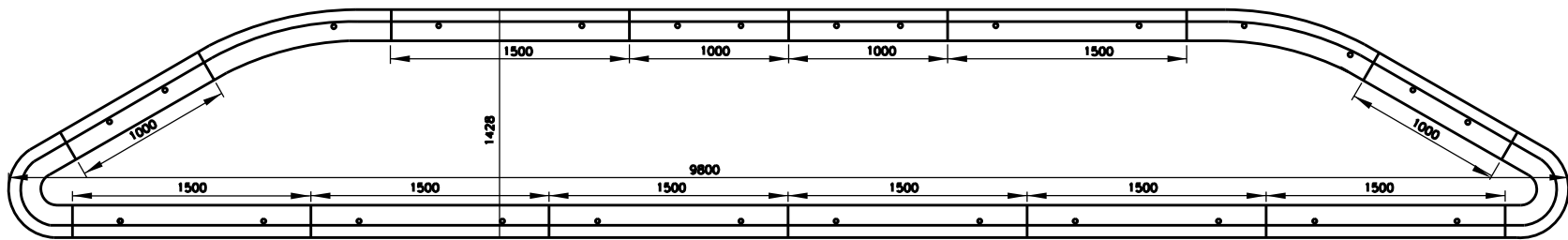
CURBSTONE ISLAND - TYPE B
