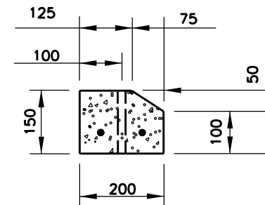
CROSS-SECTION (TYP)
