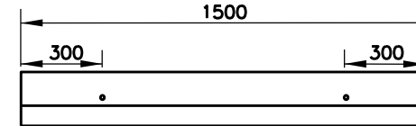
PLAN - LOCATION OF VOIDS IN EACH LENGTH
