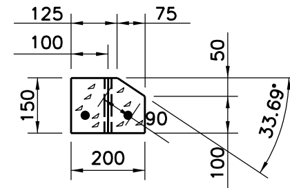
CROSS-SECTION (TYP)
