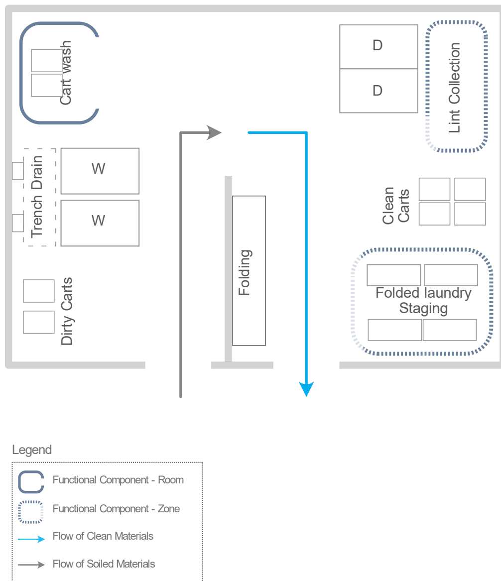
Figure 61: Diagram showing On-Premise Laundry spaces and flow of materials
