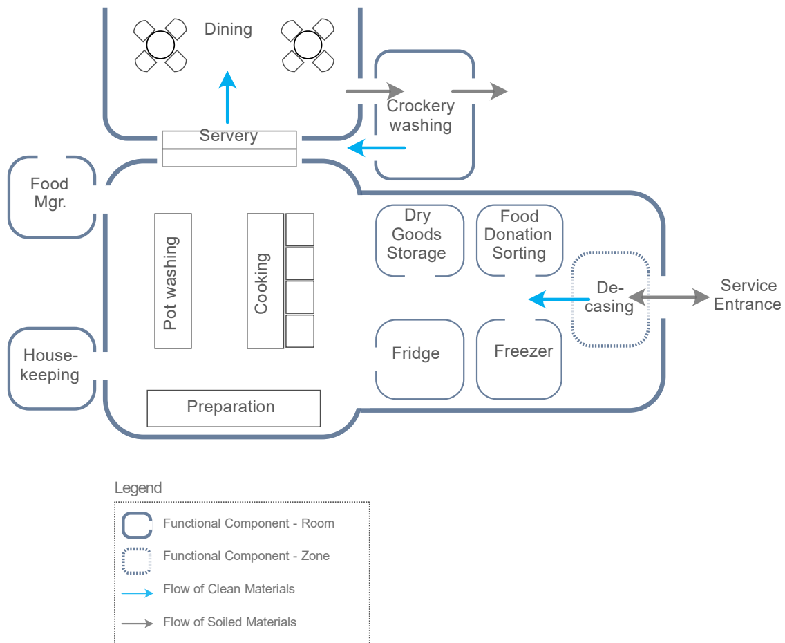
Figure 59: Diagram showing Commercial Kitchen spaces and flow of materials
