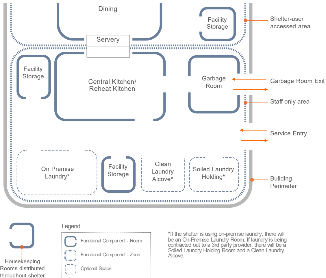
Figure 58: Diagram showing Facilities Support Spaces
