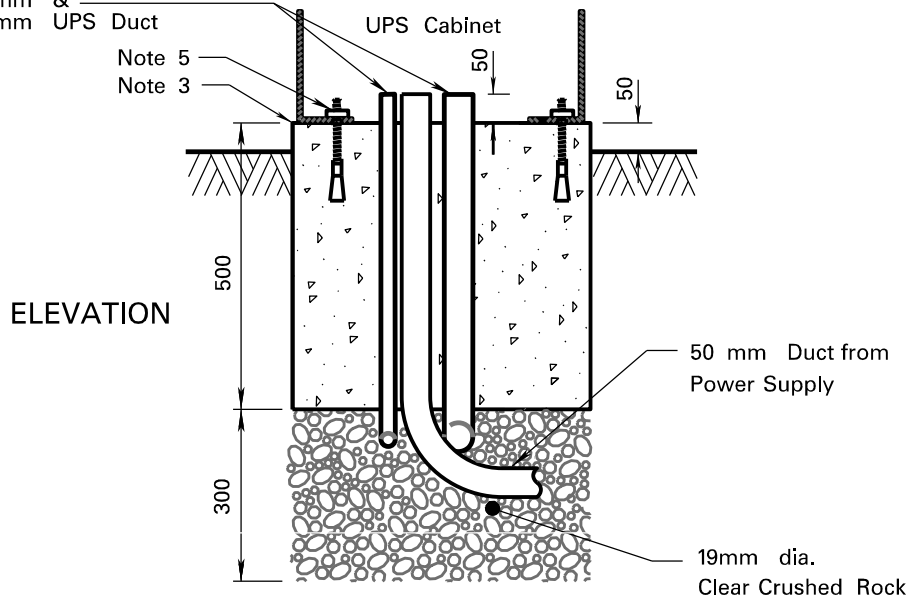
FIGURE 2 CONCRETE FOOTING FOR UPS SIDE-BY-SIDE NEW INSTALLATION
