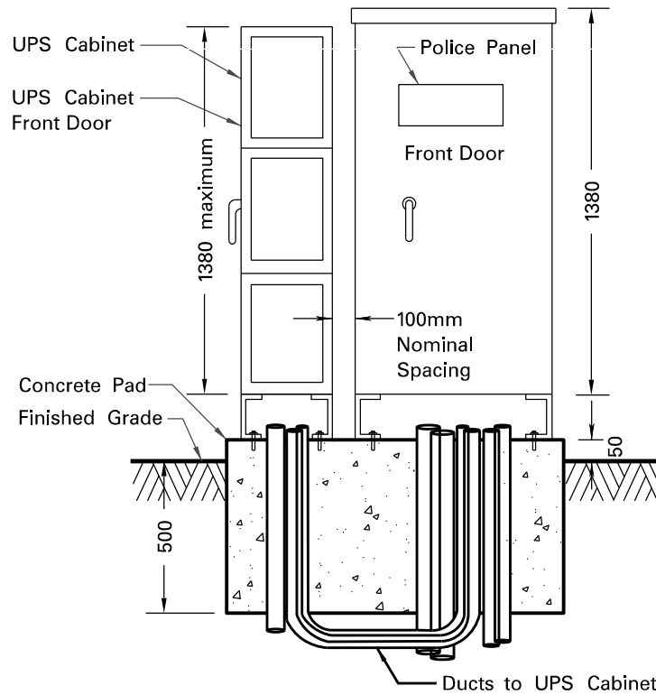
SECTION SIDE-BY-SIDE NEW INSTALLATION
