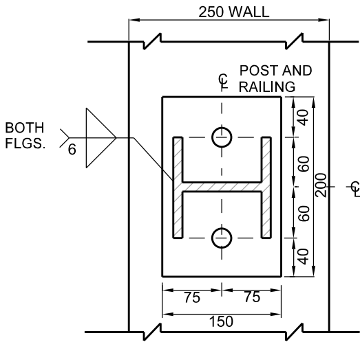
POST DETAIL
