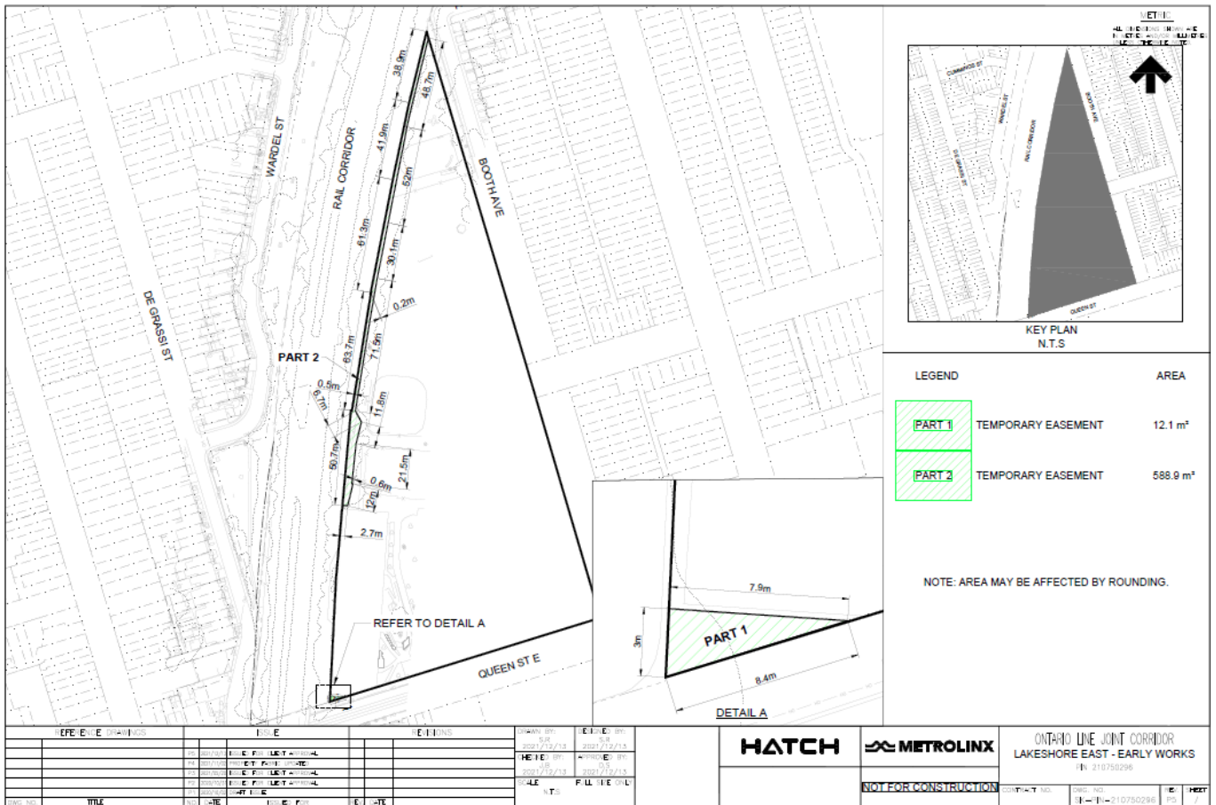
Part of 870 Queen Street East (Parts 1 & 2 on Dwg. No. SK-PIN-210750296)
