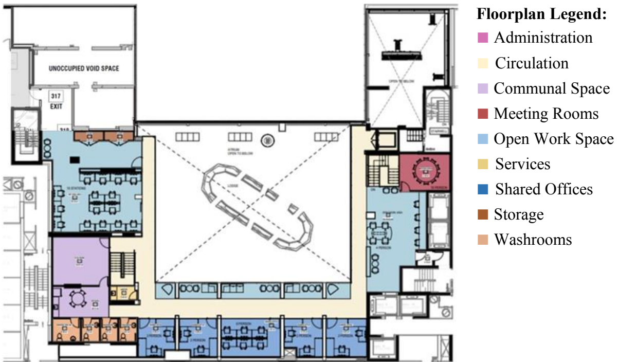
Third Floorplan
