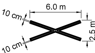
DETAIL OF PEDESTRIAN CROSSOVER "X"
