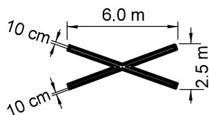
DETAIL OF PEDESTRIAN CROSSOVER "X"
