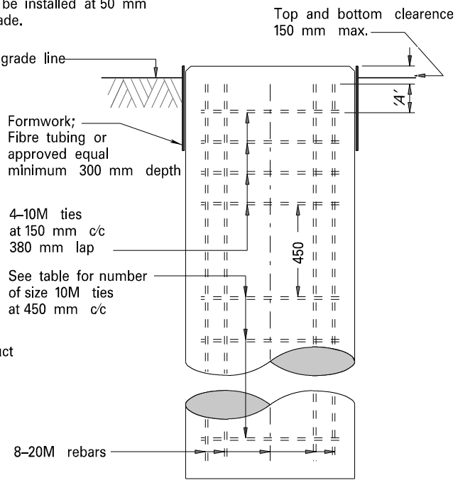
ELEVATION REINFORCEMENT
