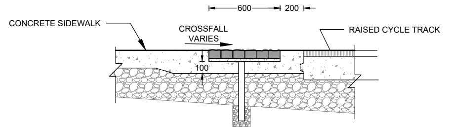
DETAIL 2 - CONCRETE CURB EDGE BETWEEN PAVERS AND CYCLE TRACK ONLY (SEE NOTE 5)
