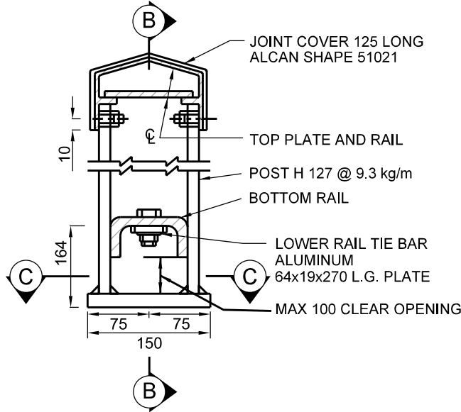
POST DETAIL
