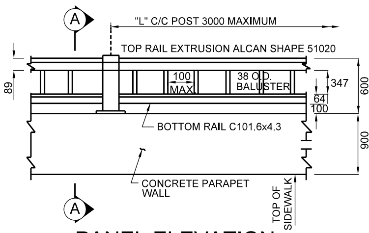
PANEL ELEVATION
