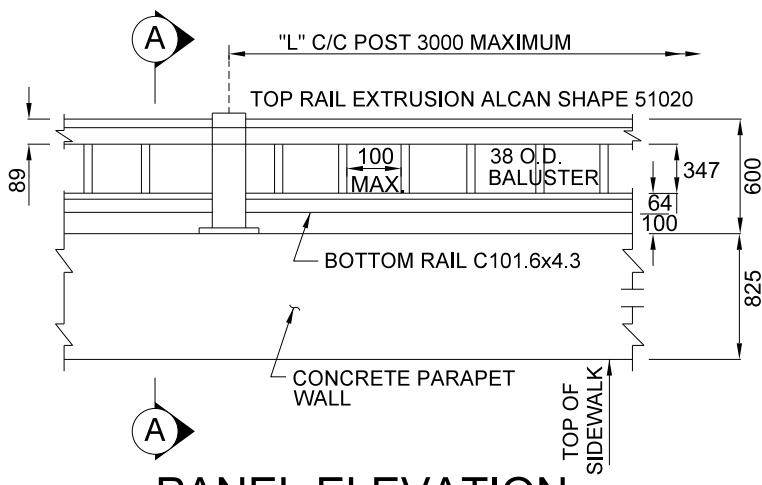
PANEL ELEVATION
