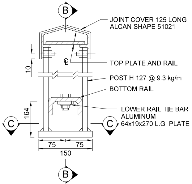
POST DETAIL
