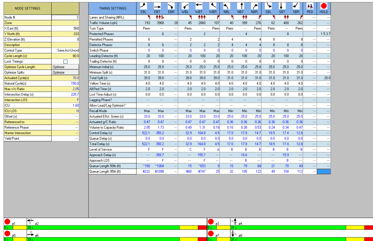
Figure 10-2 Ring structure for LPIs in Synchro
