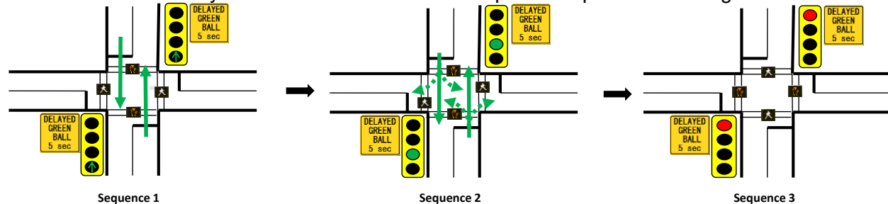
Figure 10-4: Leading Through Interval (LTI) Sequence
