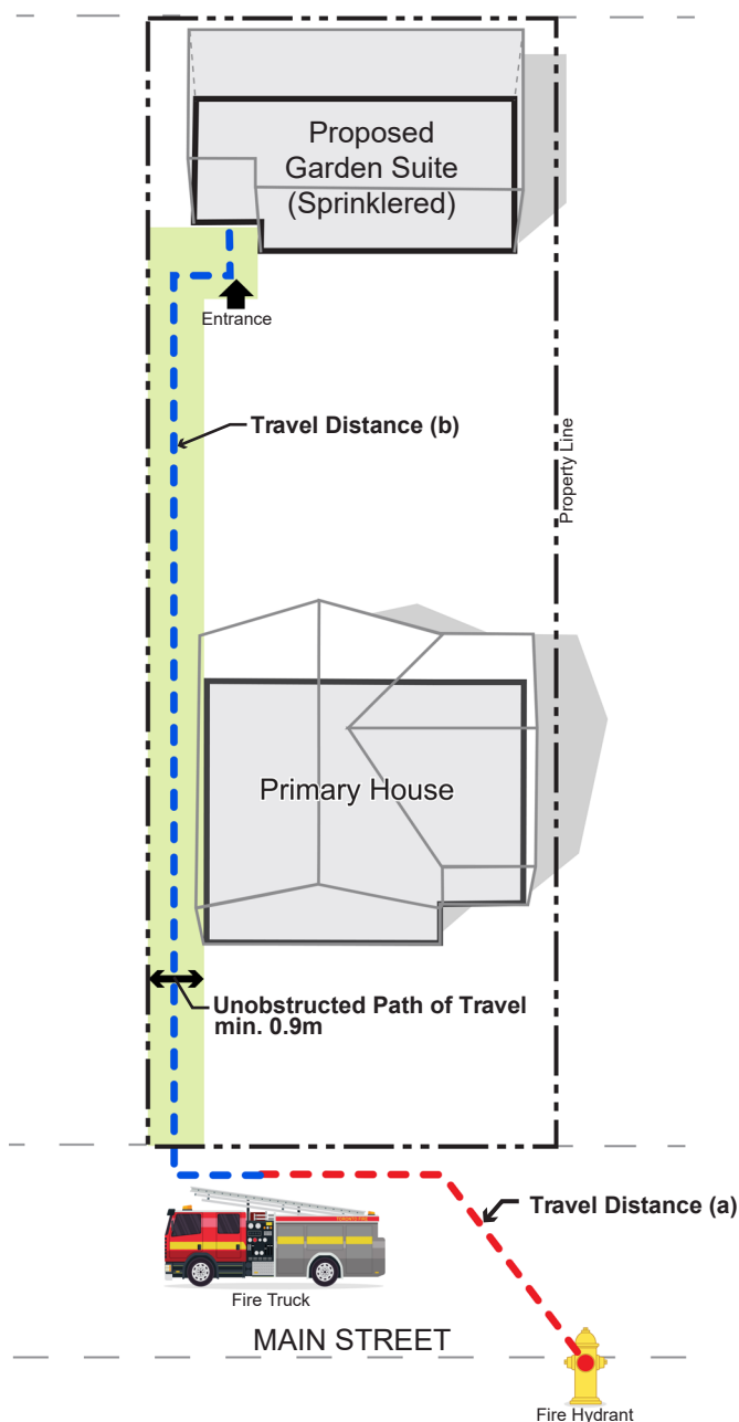
Figure 1: Fire Department Access-Sprinklered
