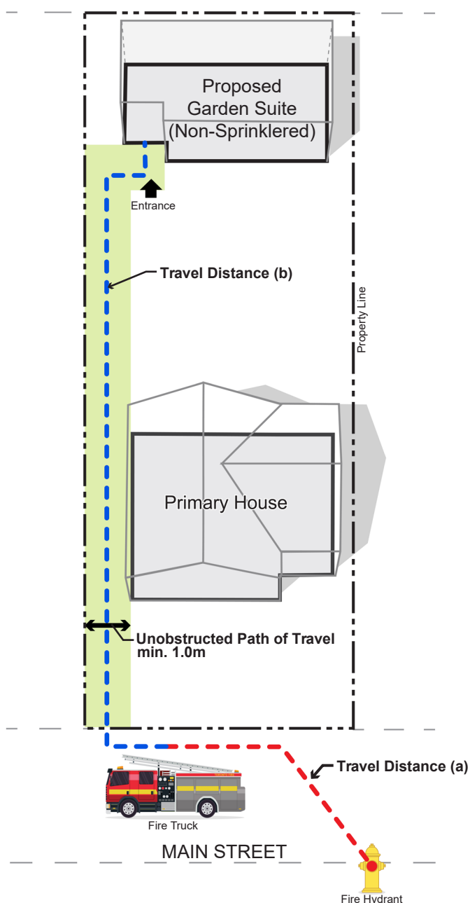
Figure 2: Fire Department Access-Non-Sprinklered
