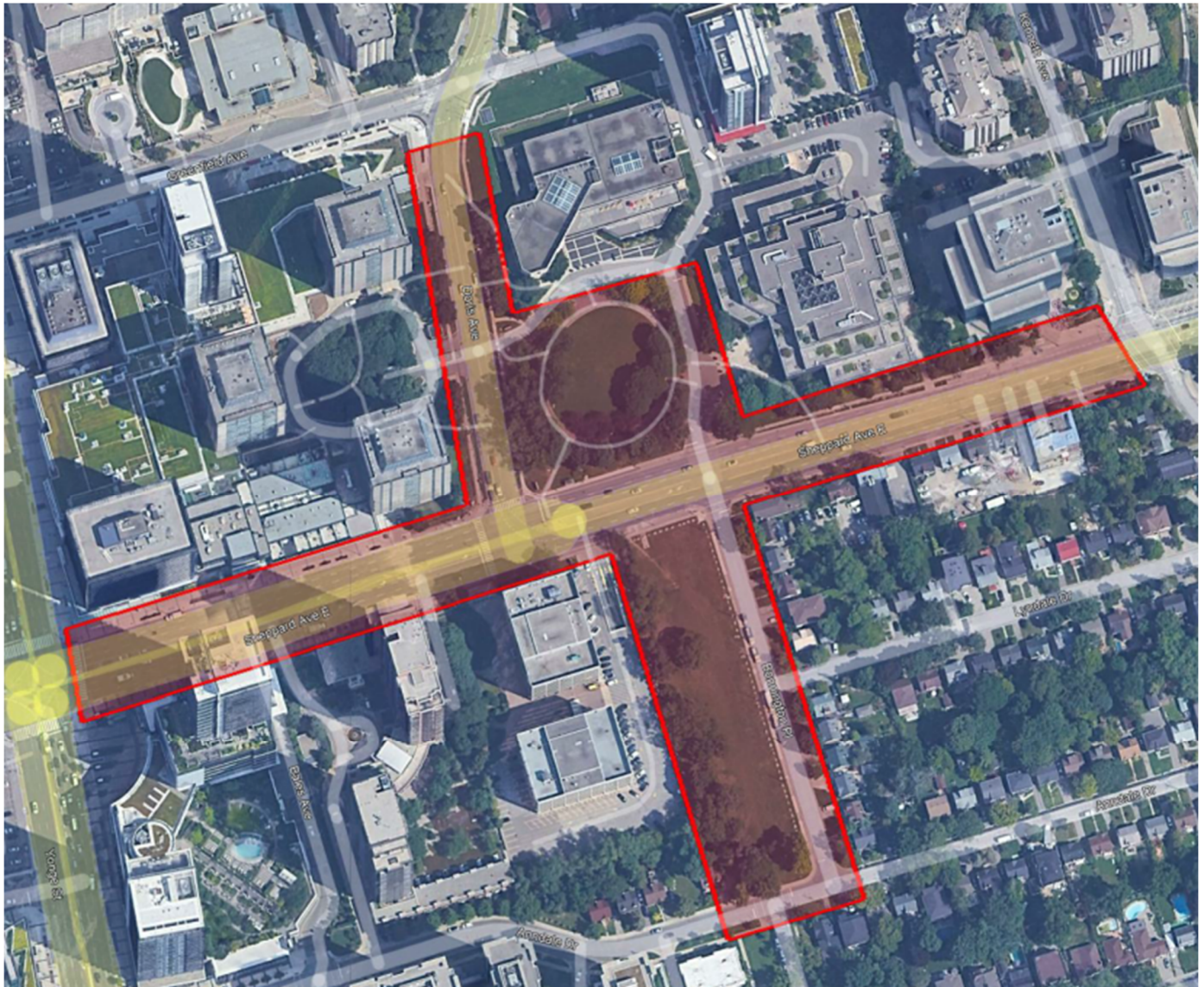
Figure 1: Outlines in red the subsurface utility investigation extent.
