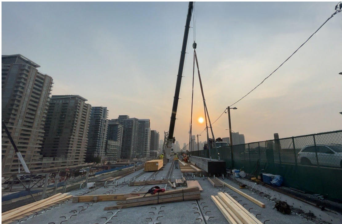
Stage 3 Girder Erection
