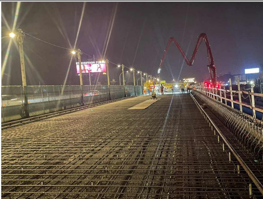
Stage 3 Bridge Deck Concrete Placement
