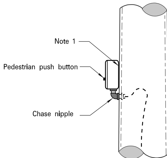
MOUNTING ON STEEL POLE
