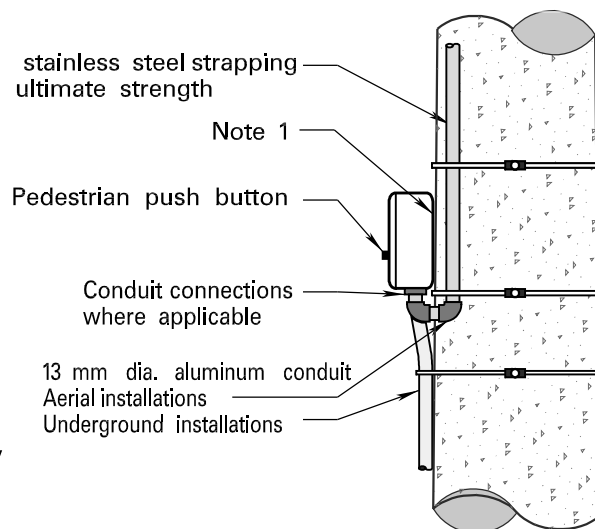
MOUNTING ON CONCRETE POLE (OTHERS)
