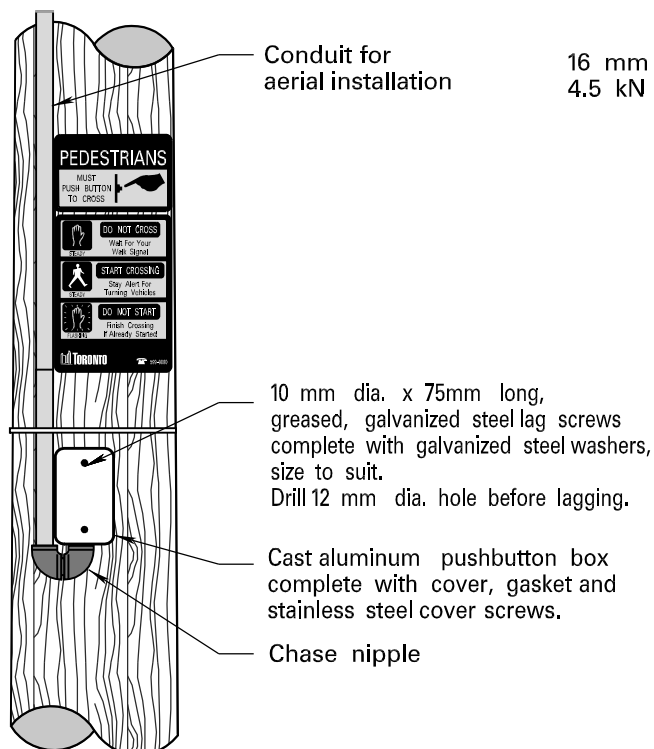
MOUNTING ON WOOD POLE OR TRAFFIC POLE
