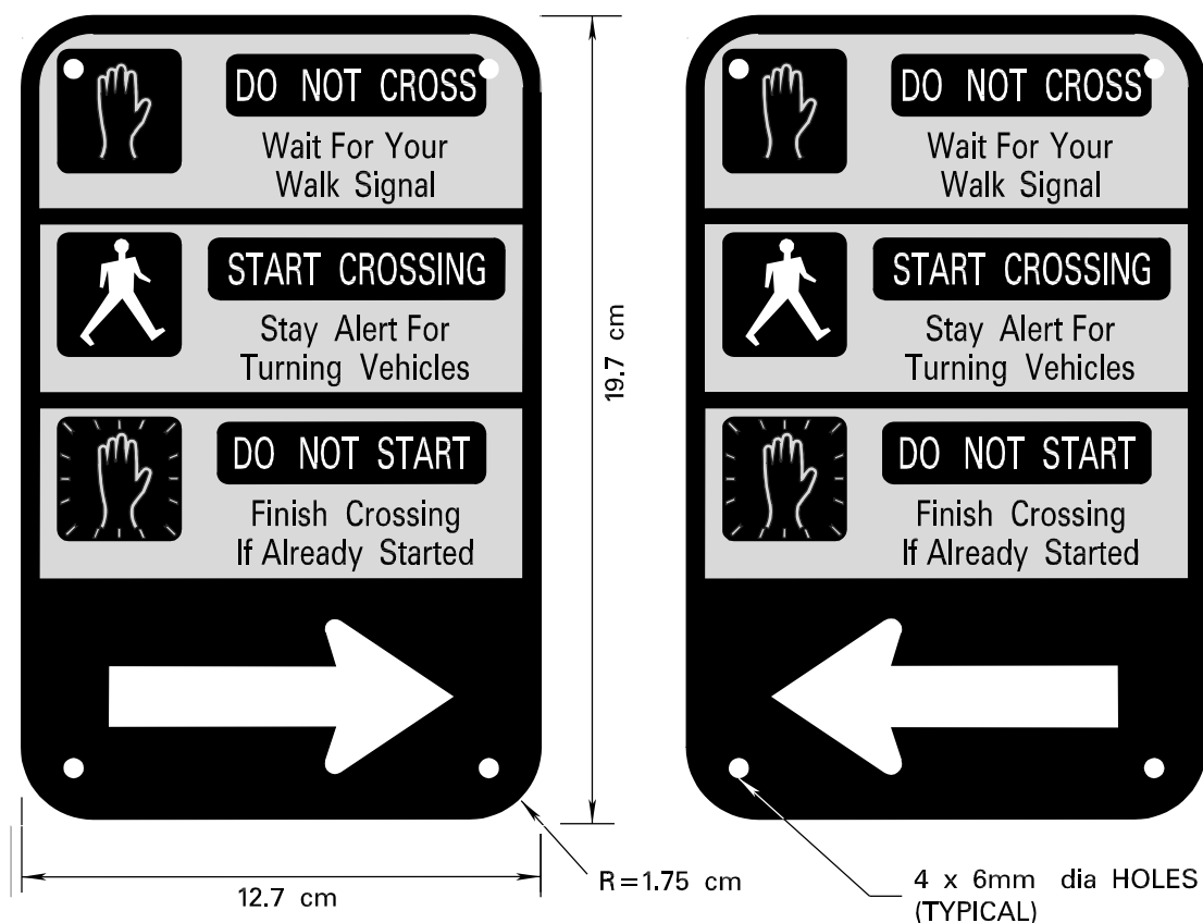
TM6010 HELPING HAND DISPLAY (RIGHT)
