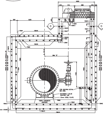
SECTION (B)
