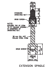
EXTENSION SPINDLE
