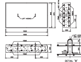
REMOVABLE SLAB
