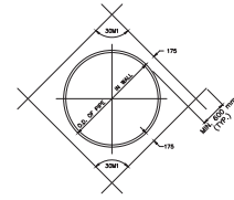
REINFORCING AROUND PIPE
