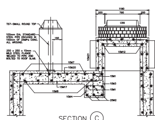
SECTION (C)
