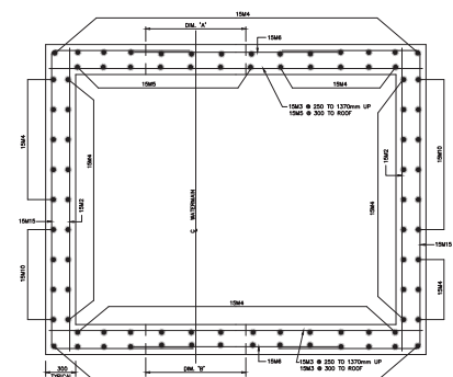
WALL SECTION
