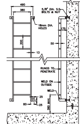
REMOVABLE ALUMINUM LADDER
