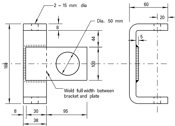
BRACKET 'A'
