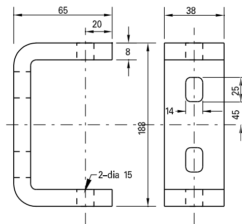
BRACKET 'C'
