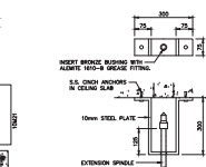
SPINDLE GUIDE BRACKET DETAIL
