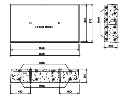
SLAB DETAIL
