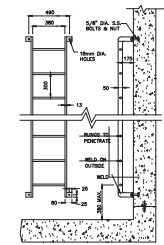
REMOVABLE ALUMINUM LADDER
