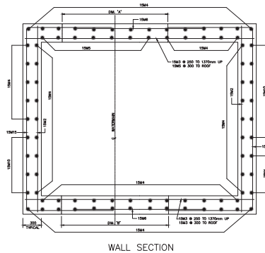
WALL SECTION
