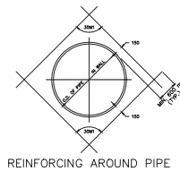
REINFORCING AROUND PIPE
