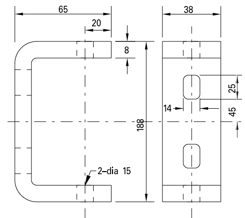
BRACKET 'C'
