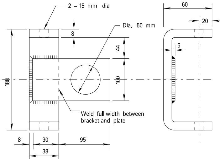
BRACKET 'A'
